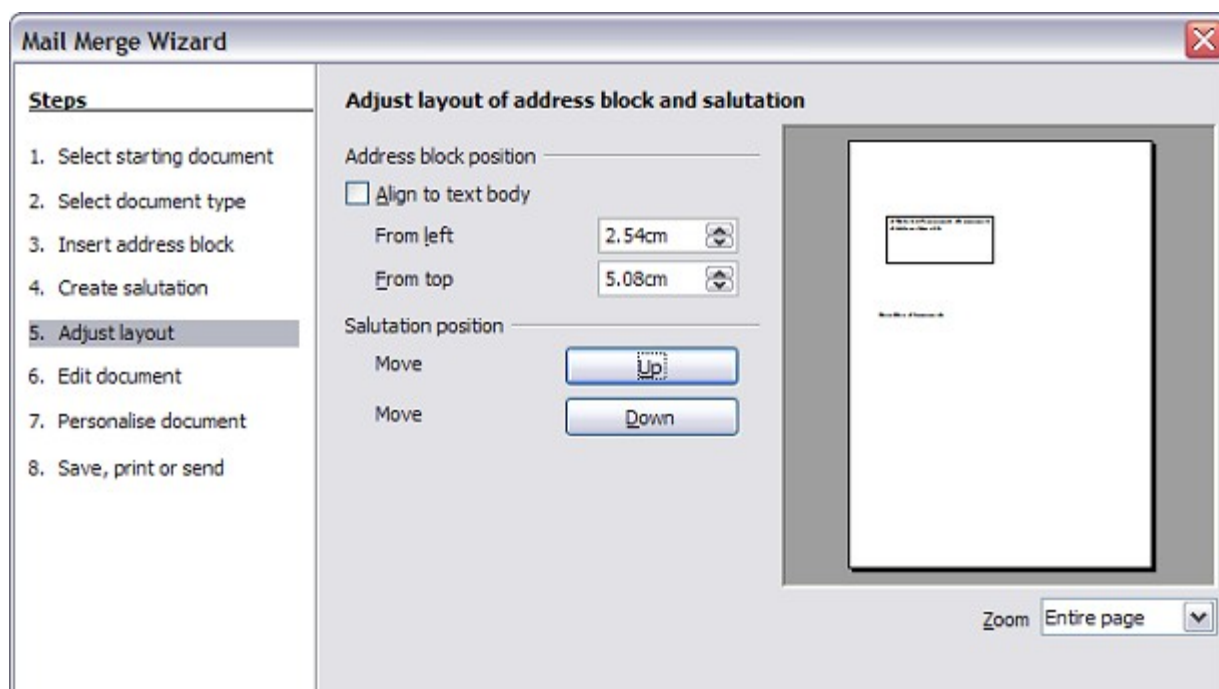
Figure 316: Adjust layout
