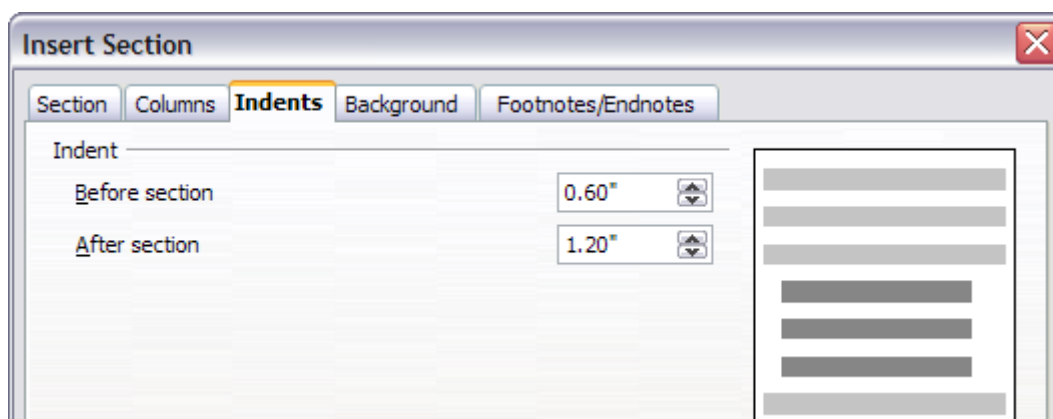
Figure 124: Indenting sections
