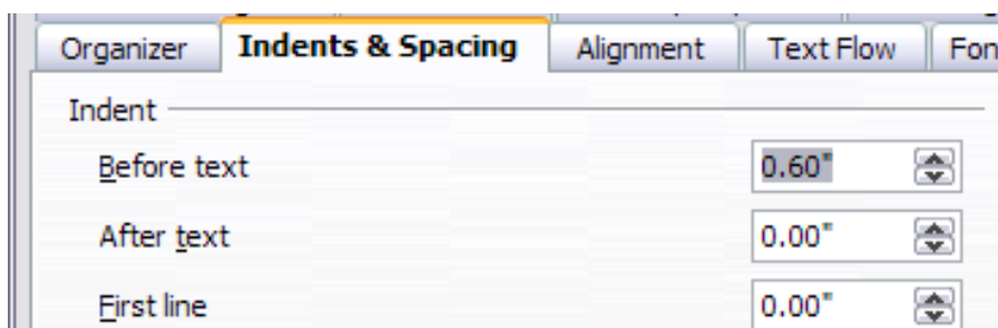
Figure 188: Set indentation
