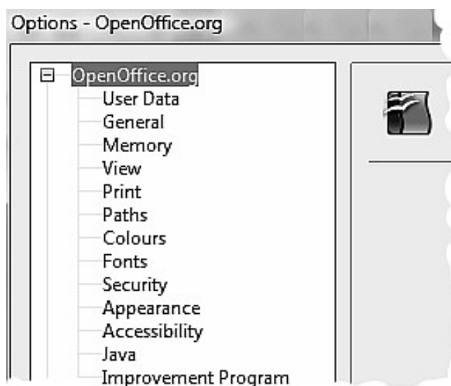
Figure 22: OpenOffice.org options
