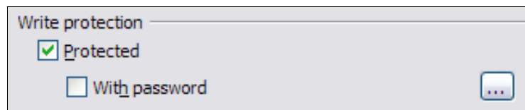
Figure 121: Write-protecting sections
