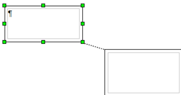
Figure 111: Linked frames
