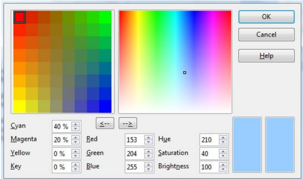
Figure 31: Editing colors
