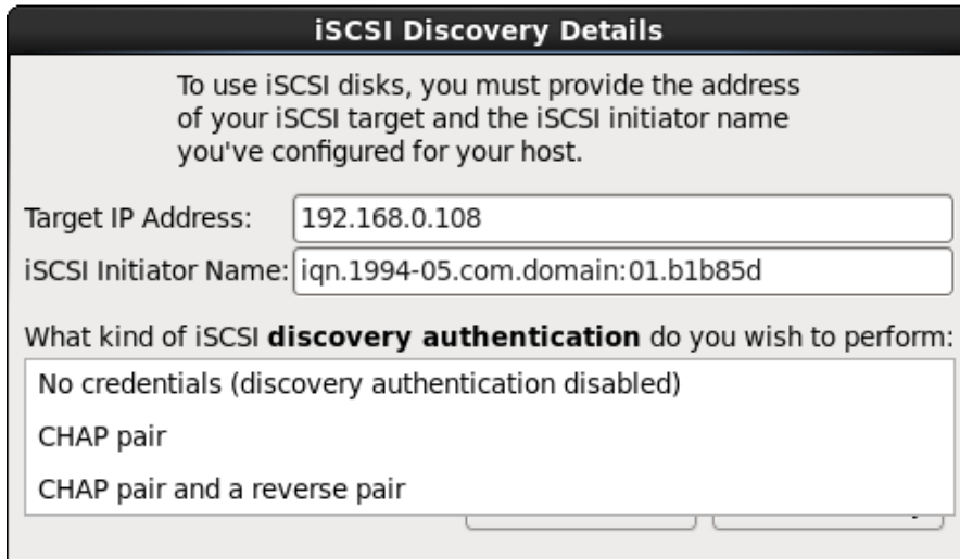
Figure 23.12. iSCSI discovery authentication
