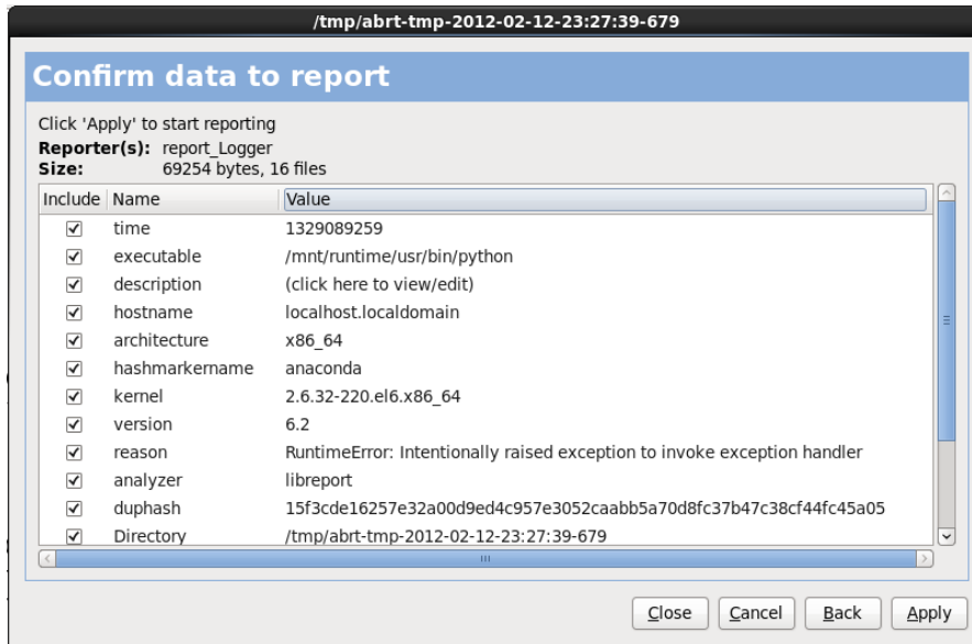
Figure 17.9. Confirm report data
