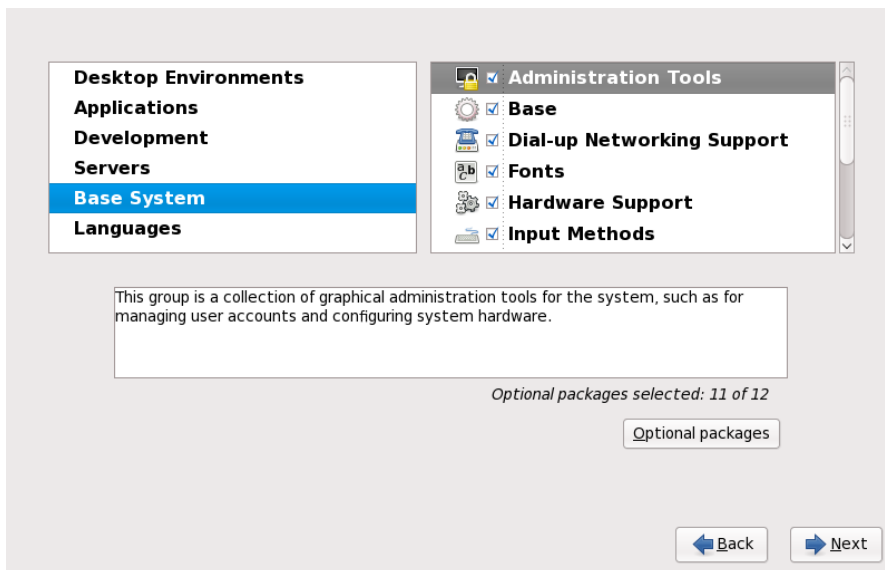
Figure 23.50. Package Group Details
