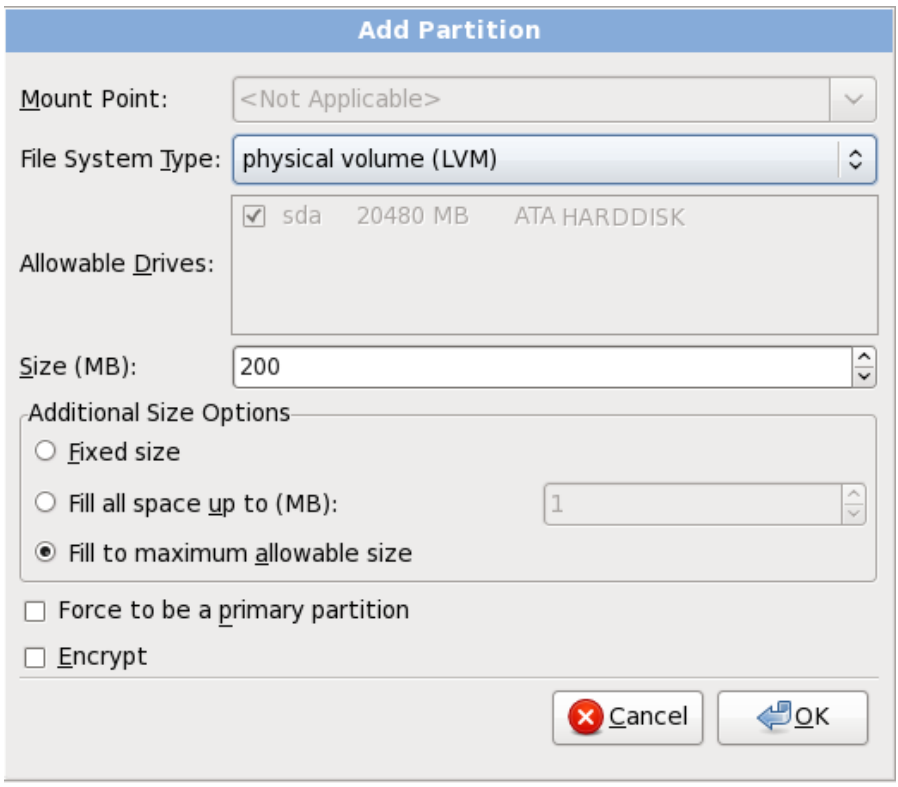
Figure 16.43. Create an LVM Physical Volume
