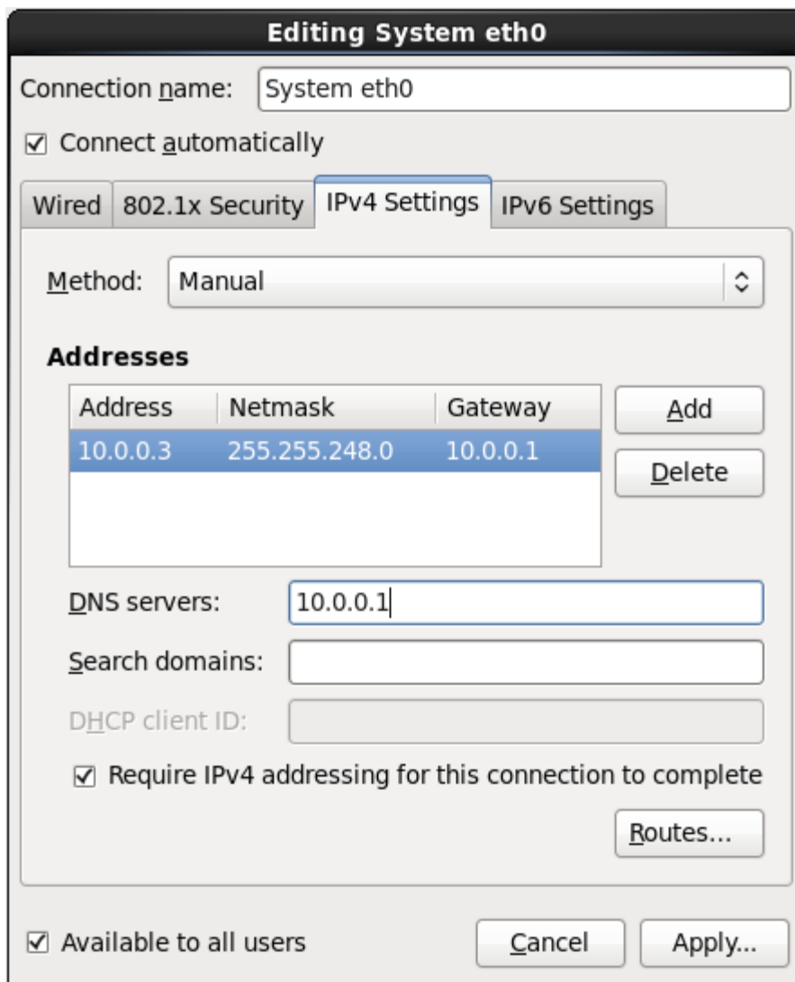
Figure 16.27. The IPv4 Settings tab
