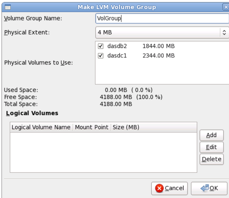
Figure 23.43. Make LVM Volume Group
