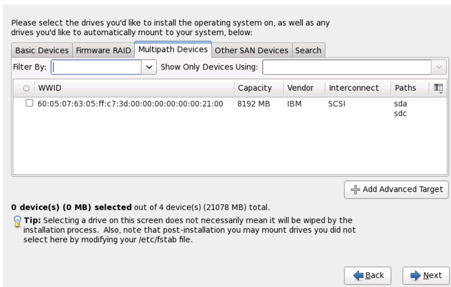
Figure 9.5. Select storage devices — Multipath Devices
