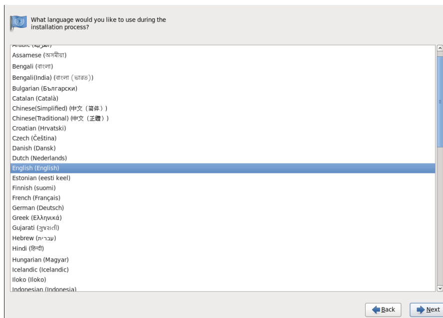
Figure 16.1. Language Configuration
