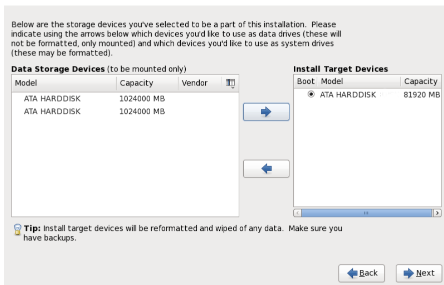
Figure 16.33. Assign storage devices
