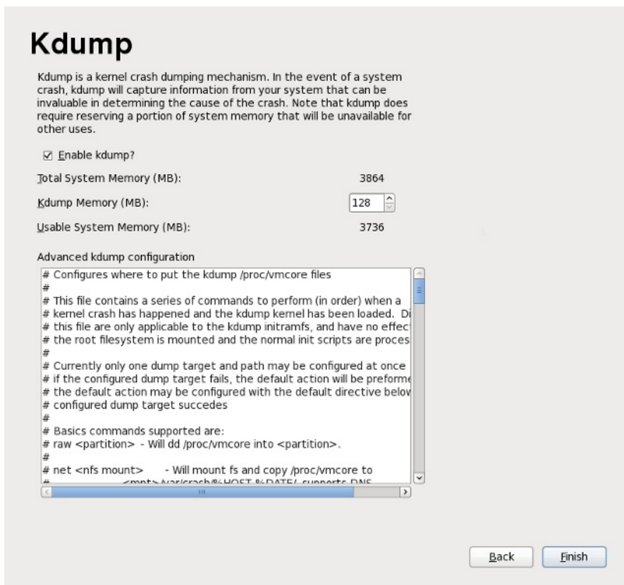
Figure 34.21. Kdump enabled
