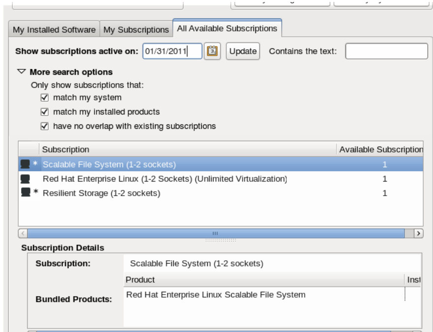
Figure 34.10. Selecting subscriptions
