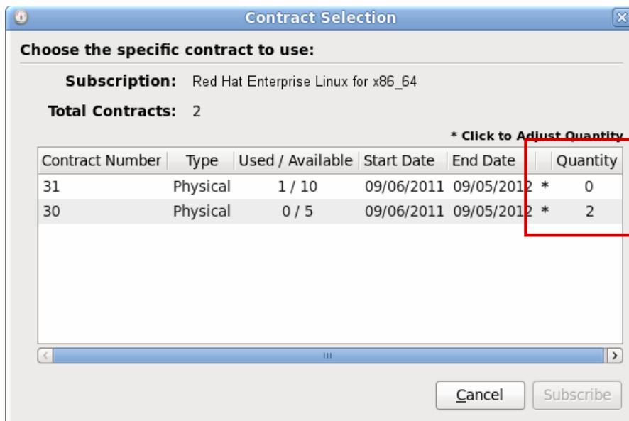
Figure 34.11. Setting Quantities
