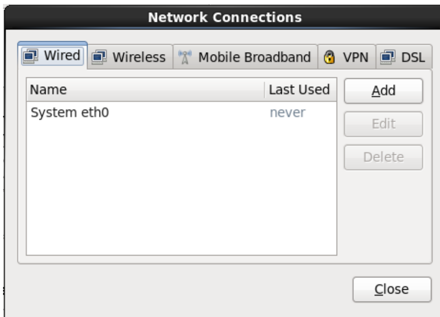
Figure 9.53. Network Connections
