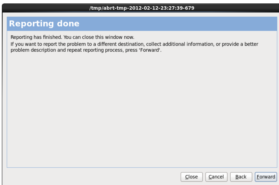
Figure 24.11. Reporting done
