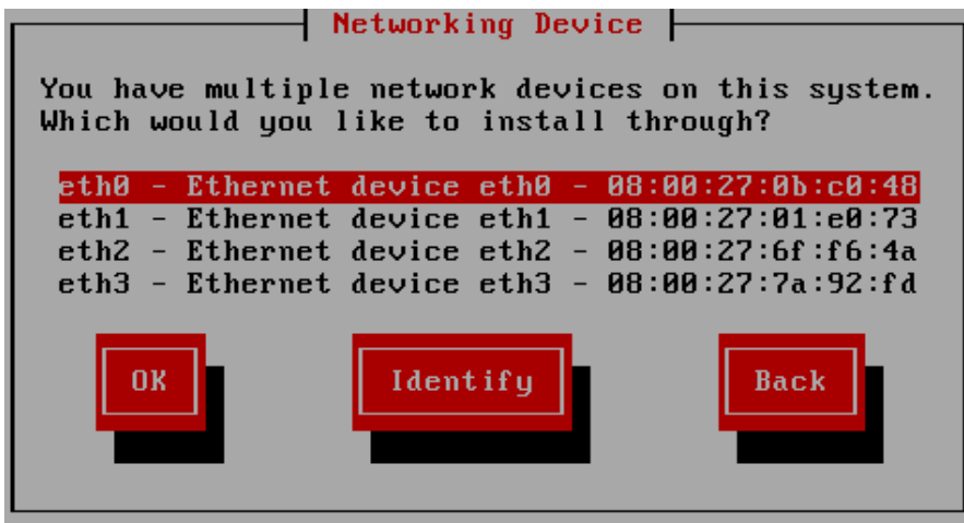
Figure 15.6. Networking Device
