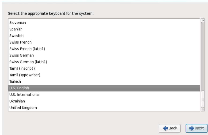
Figure 16.2. Keyboard Configuration
