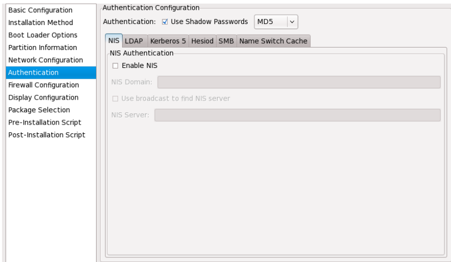
Figure 33.9. Authentication
