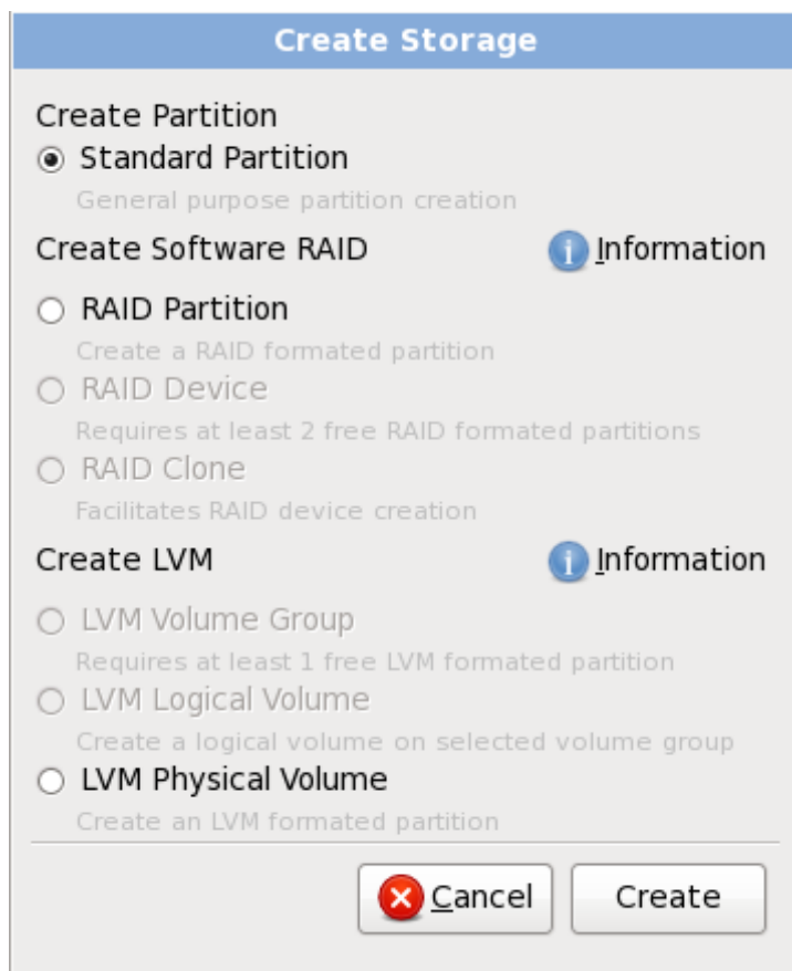
Figure 9.40. Creating Storage
