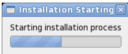
Figure 9.56. Starting installation
