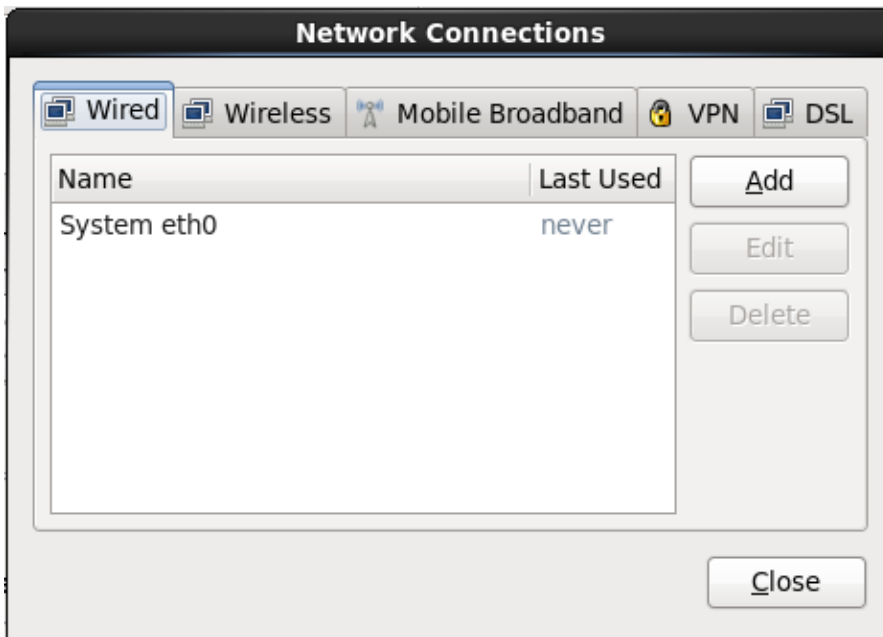
Figure 23.23. Network Connections
