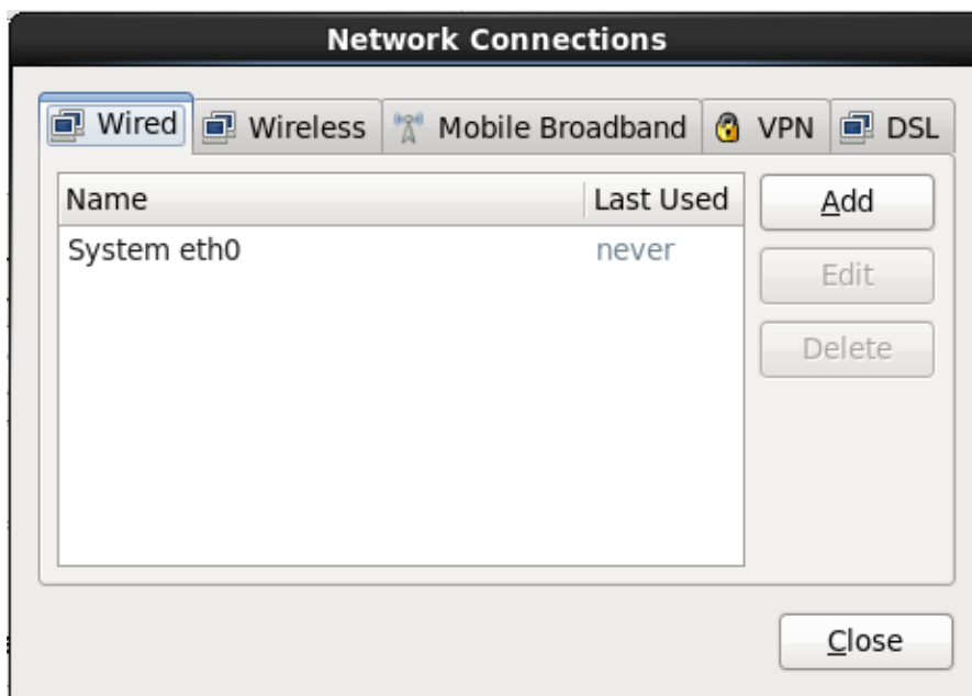
Figure 16.50. Network Connections
