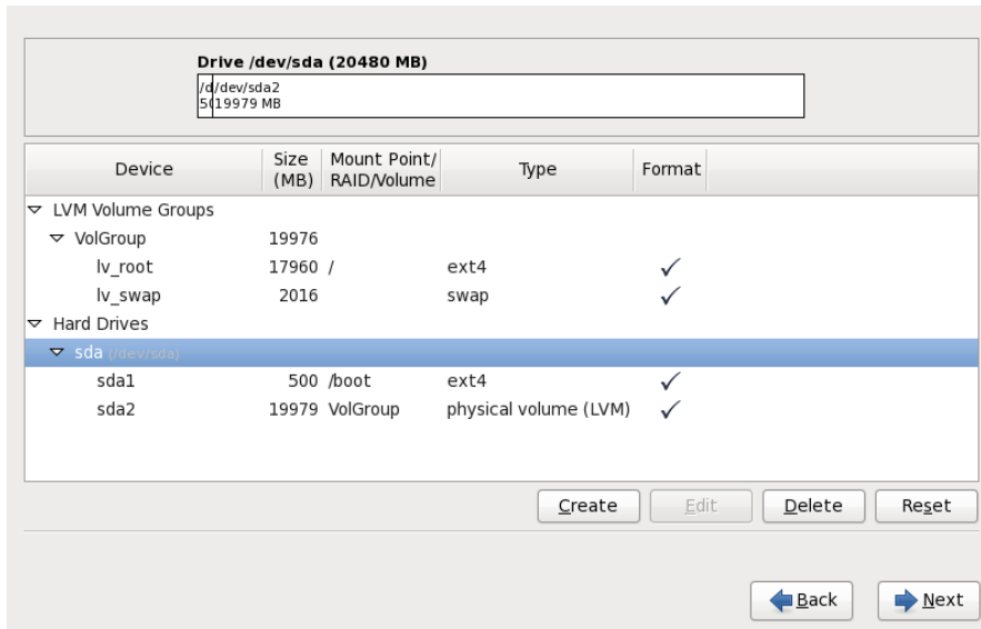
Figure 9.39. Partitioning on x86, AMD64, and Intel 64 Systems
