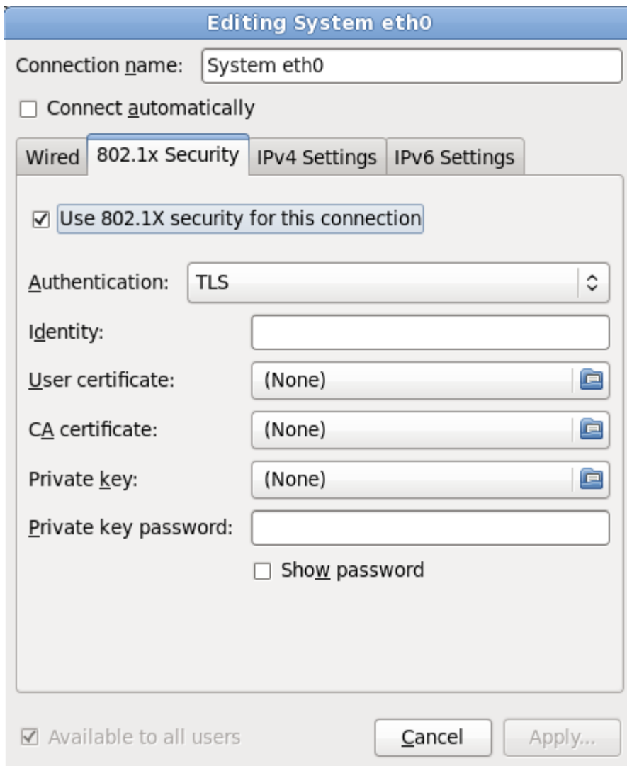
Figure 9.26. The 802.1x Security tab
