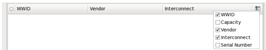
Figure 9.8. Selecting Columns
