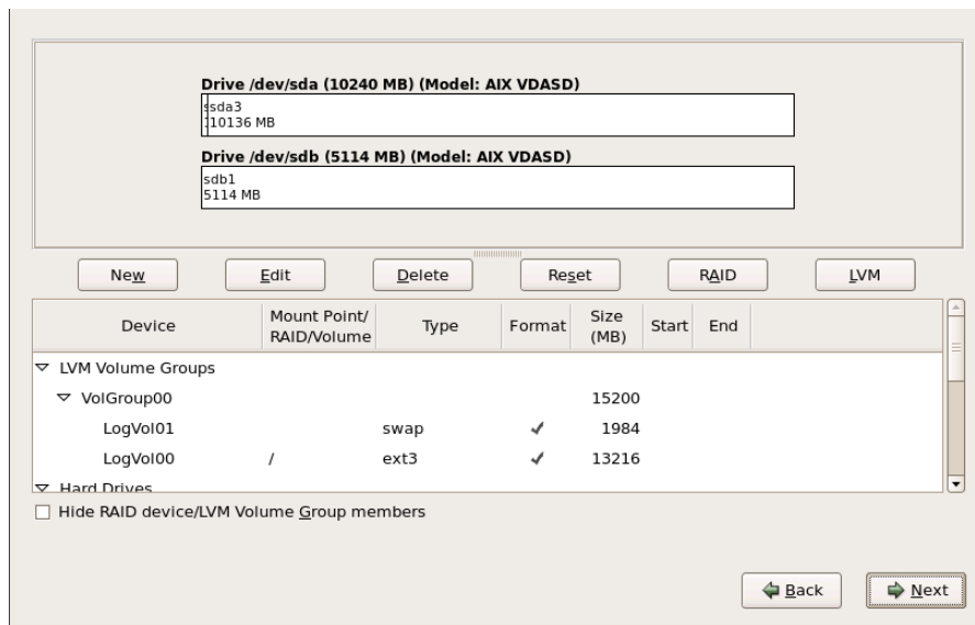
Figure 16.38. Partitioning on IBM System p
