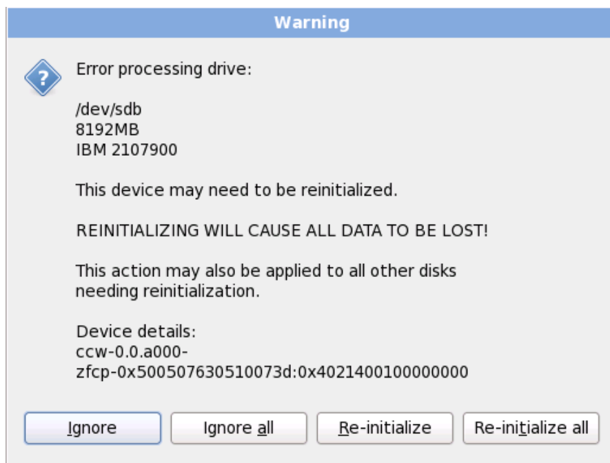
Figure 23.34. Warning screen – initializing FCP LUN
