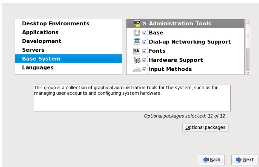
Figure 16.51. Package Group Details
