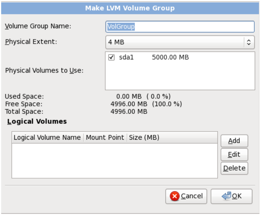
Figure 16.44. Make LVM Volume Group
