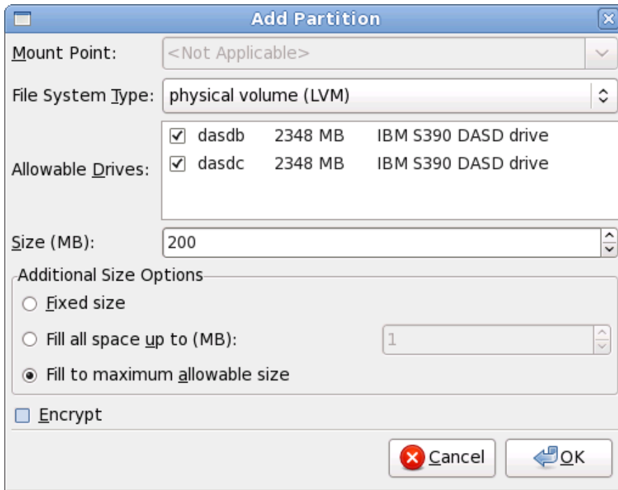
Figure 23.42. Create an LVM Physical Volume
