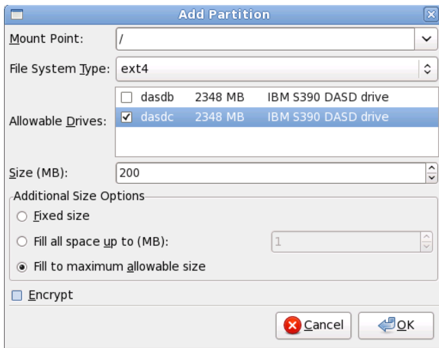
Figure 23.39. Creating a New Partition
