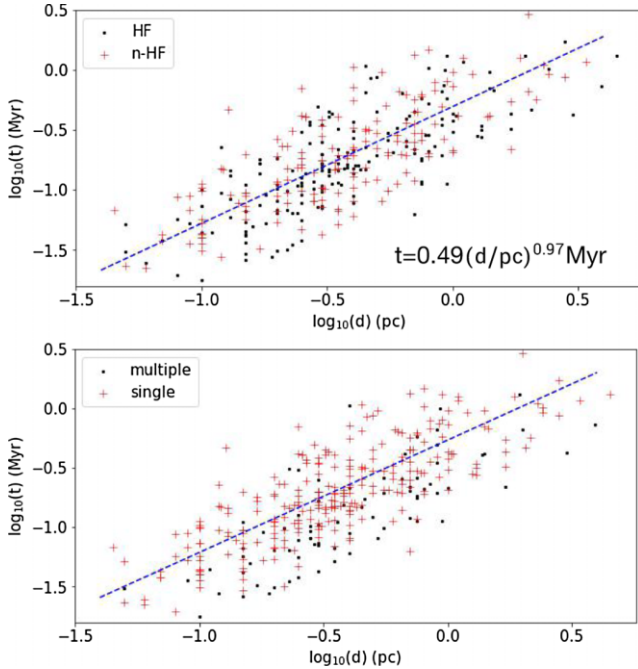
Figure 11. Gas accretion time-scale t_{\text{inflow}} versus filament length d_{\text{fila}} over which the velocity gradient is estimated. (a) HFS (black dots) and non-HFSs (red crosses); (b) sources (red crosses) showing singly peaked profiles of \text{H}^{13}\text{CO}^+ line emission in hub regions and sources (black dots) showing multiple-peaked profiles.
