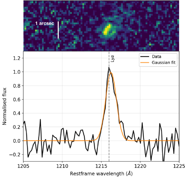
Figure 6. Rest-frame 1D spectrum showing the asymmetric \text{Ly}\alpha line profile at a redshift of z = 5.720 . Also shown is the best-fit Gaussian to the emission line. The peak of the fitted Gaussian is slightly redder than the peak of the line, suggesting asymmetry in the emission line. This is also clear from the excess towards the redder parts of the Gaussian. Top: The 2D GMOS spectrum showing the detected \text{Ly}\alpha line. The spatial extent of the emission is roughly 1 arcsec, which is also the aperture size used to extract the 1D spectrum.
