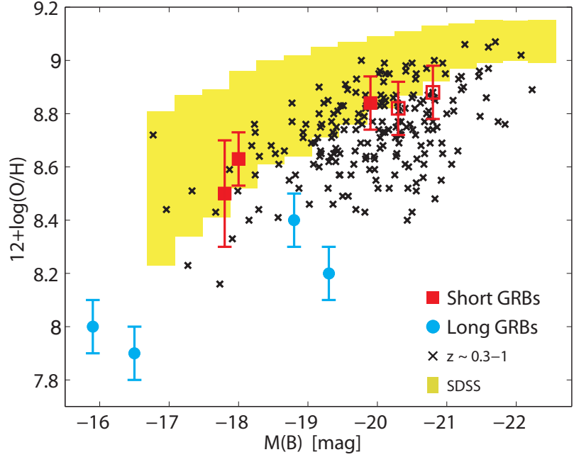
Figure 12 Metallicity as a function of B -band absolute magnitude for the host galaxies of short (red) and long (blue) GRBs. The yellow bars mark the 14 – 86 percentile range for galaxies at z \sim 0.1 from the Sloan Digital Sky Survey (Tremonti et al. 2004), while crosses designate field galaxies at z \sim 0.3 - 1 (Kobulnicky and Kewley 2004). Both field samples exhibit a clear luminosity-metallicity relation. The long GRB hosts tend to exhibit lower than expected metallicities (Stanek et al. 2006), while the hosts of short GRBs have higher metallicities by about 0.6 dex and are moreover in excellent agreement with the luminosity-metallicity relation. From Berger (2009).
