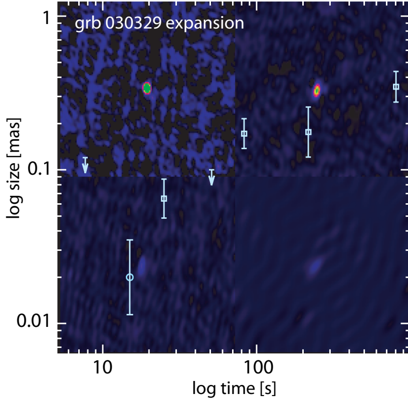
Figure 8 The growth of GRB 030329 with time as measured using VLBI (by Pihlström et al. 2007 and references therein). In the background are the images from (a) April 2003 (15 GHz), (b) June 2003 (8 GHz), (c) November 2003 (8 GHz), and (d) June 2005 (5 GHz) with the same intensity scale. The resolution for the four images is not constant in time, but is accounted for in the analysis of the source size.
