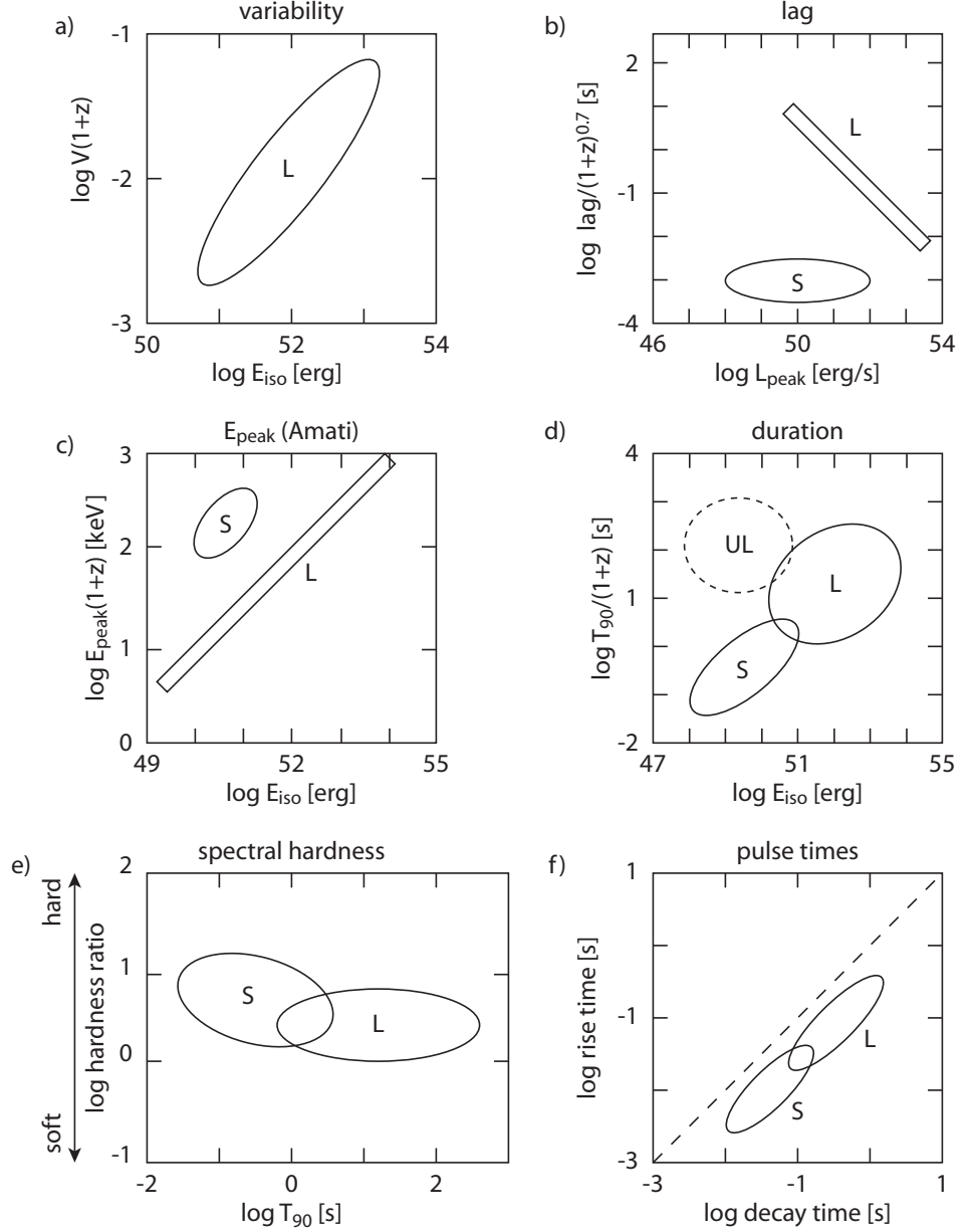
Figure 5 Schematic diagrams illustrating the most widely discussed correlations between various prompt emission properties for long (L), short (S), and underluminous (UL) GRBs. (a) Variability scaled to the burst frame versus E_{\text{iso}} (Fenimore and Ramirez-Ruiz 2000, Reichart et al. 2001, Schaefer 2006). The variability is a measure of the spikiness of the lightcurve and is defined as the mean square of the time signal after removing low frequencies by smoothing. (b) Spectral lag scaled to the burst frame versus peak luminosity (Norris and Bonnell 2006; Gehrels et al. 2006). (c) E_{\text{peak}} scaled to the burst frame versus E_{\text{iso}} (Amati et al. 2002 for BeppoSAX GRBs; Amati 2006 for Swift GRBs; Lloyd-Ronning and Ramirez-Ruiz 2002 for BATSE events). (d) Duration scaled to the burst frame versus E_{\text{iso}} . (e) Spectral hardness versus observed duration (Kouveliotou et al. 1993). (f) Pulse rise time versus its decay time (Norris et al. 1996).
