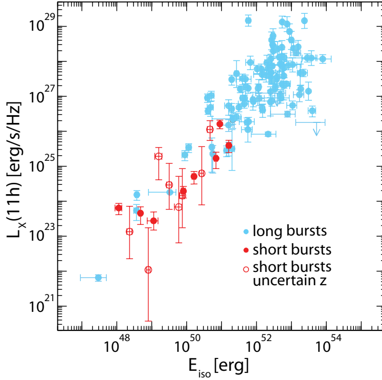
Figure 9 Isotropic-equivalent luminosity of GRB X-ray afterglows scaled to t = 11 hr (5 keV source frame) after the burst trigger as a function of their isotropic \gamma -ray energy release (adapted from Nysewander et al. 2008).
