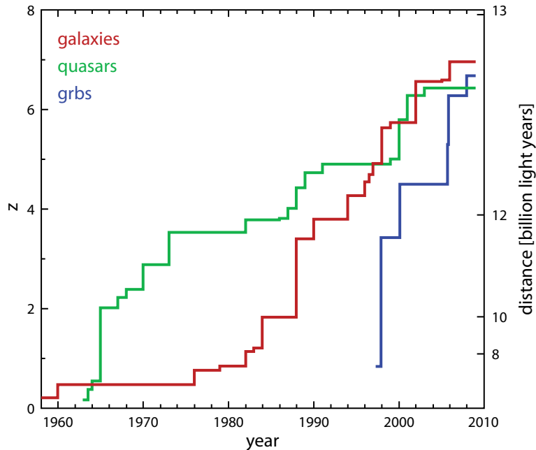
Figure 16 High- z record holders. The history of most distant objects detected in categories of galaxies, quasars, and GRBs (R. McMahon, N. Tanvir, priv. comm.).
