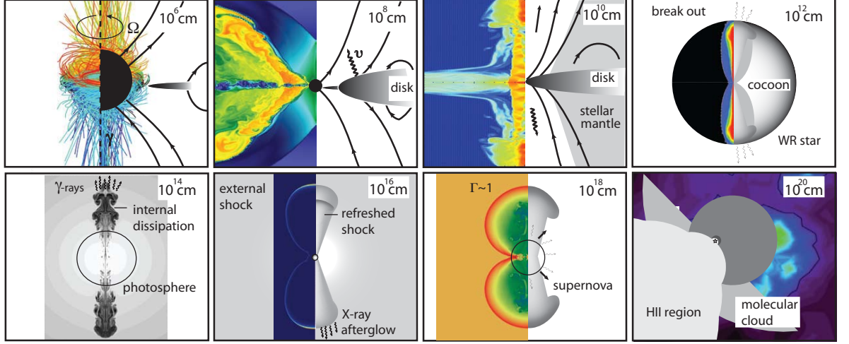
Figure 14 Diagram exhibiting GRB activity over successive decades in radius ranging from 10^6 cm to 1pc. The first task in attempting to construct a general scheme of GRBs is to decide which parameters exert a controlling influence upon their properties. ( 10^6 cm) The GRB nucleus (BH or NS) and its magnetosphere. ( 10^8 cm) The accretion flow is likely to be embedded in a very active corona. We expect coronal arches, as well as large magnetic structures, to be quite common and to be regenerated on an orbital timescale. Relativistic outflow from the black hole is proposed to be focused into two jets. ( 10^{10} cm) Even if the outflow is not narrowly collimated, some beaming is expected because energy would be channelled preferentially along the rotation axis. The majority of stellar progenitors, with the exception of some very compact stars, will not collapse entirely during the typical duration of a GRB. A stellar envelope will thus remain to impede the advance of the jet. ( 10^{12} cm) This is the typical size of an evolved massive star progenitor. A thermal break-out signal should precede the canonical, softer \gamma -rays observed in GRBs. ( 10^{14} cm) Velocity differences across the jet profile provide a source of free energy. The most favourable region for shocks producing highly variable \gamma -ray light curves is above the baryonic or pair-dominated photosphere. ( 10^{16} cm) The external shock becomes important when the inertia of the swept-up external matter starts to produce an appreciable slowing down of the ejecta. ( 10^{18} cm) Finally, we come to the end of the relativistic phase. This happens when the mass E/c^2 has been swept-up.
