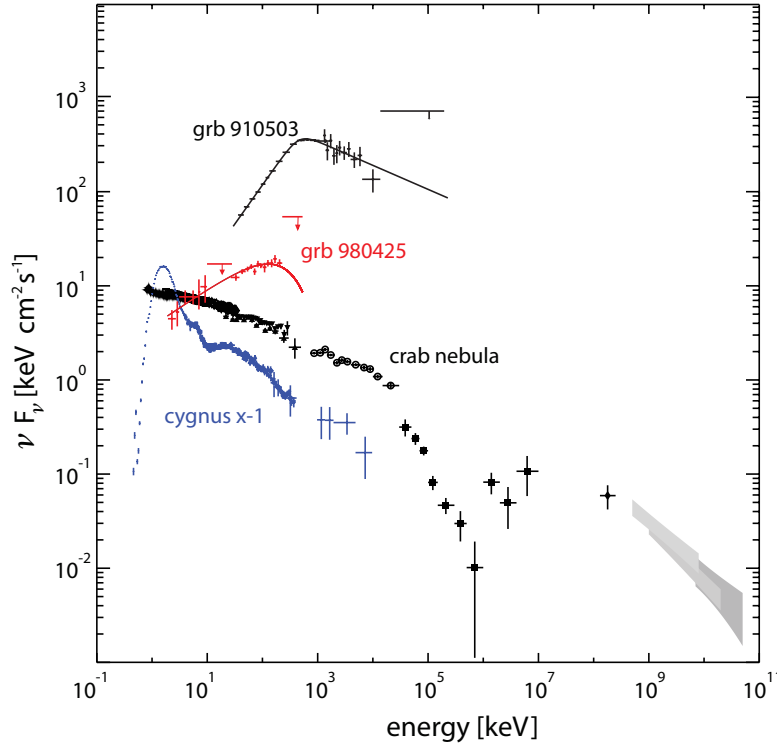
Figure 1 Gamma-rays are excellent probes of the most energetic phenomena in nature, that typically involve dynamical non-thermal processes and include interactions of high energy electrons with matter, photons and magnetic fields; high energy nuclear interactions; matter- antimatter annihilation and possibly other fundamental particle interactions. Here shown are representative spectra \nu F_\nu \propto \nu^2 N(\nu) of GRBs (Kaneko et al. 2007; Kaneko et al. 2008) together with the Crab pulsar nebula (Kuiper et al. 2001) and the galactic black hole candidate Cygnus X-1 (McConnell et al. 2002).
