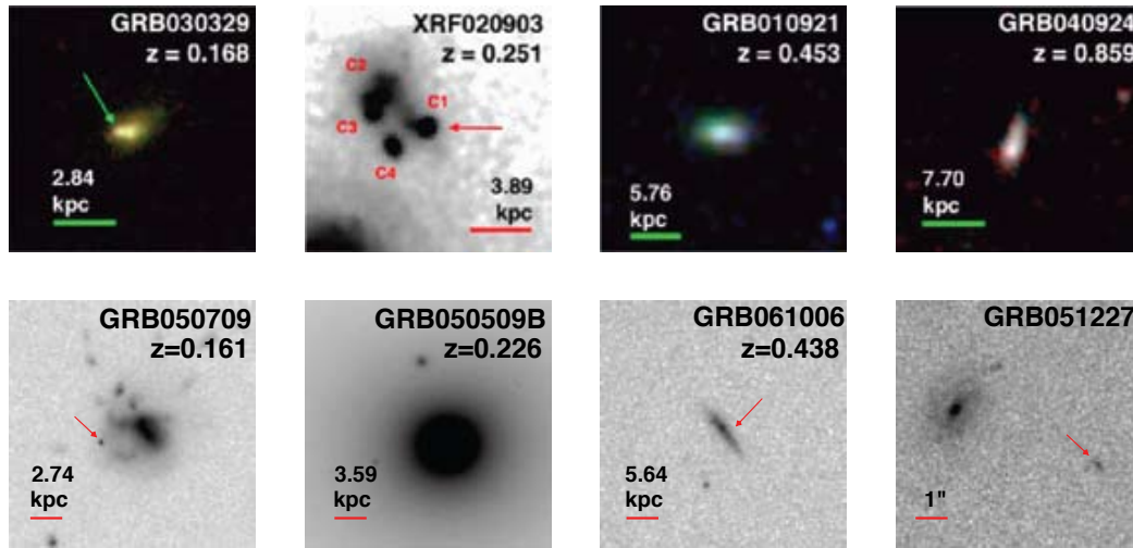
Figure 11 A selection of the host galaxies of long-duration (top row) and short-duration (bottom row) gamma-ray bursts, as imaged by the Hubble Space Telescope . An attempt has been made to choose pairs of long and short burst host galaxies with comparable redshifts; lower-redshift hosts are emphasized as these reveal their structure more readily in short exposures. Images are oriented with North up and East to the left, and the physical length scale for a one-arcsecond angular distance is indicated in each panel (except for GRB 051227); arrows point to the location of the burst where this is known to \sim pixel precision. Individual burst notes: GRB 030329 was the first classical long GRB to be associated with a well-observed spectroscopic supernova (Stanek et al. 2003, Hjorth et al. 2003); XRF 020903 was the first X-ray Flash event to yield a redshift measurement Soderberg et al. (2004); GRB 050709 was the first short burst with optical afterglow – indicated by the arrow – detected Fox et al. (2005), Hjorth et al. (2005b); GRB 050509B was the first short burst with detected afterglow (Gehrels et al. 2005; Bloom et al. 2006) GRB 051227 has a faint candidate host, of unknown redshift probably greater than 1, visible at the optical afterglow location; the spiral galaxy to the east has redshift z = 0.714 Foley et al. (2005). Long-burst host images from Wainwright et al. (2007); short-burst host images from Fox et al. (2005) and this work.
