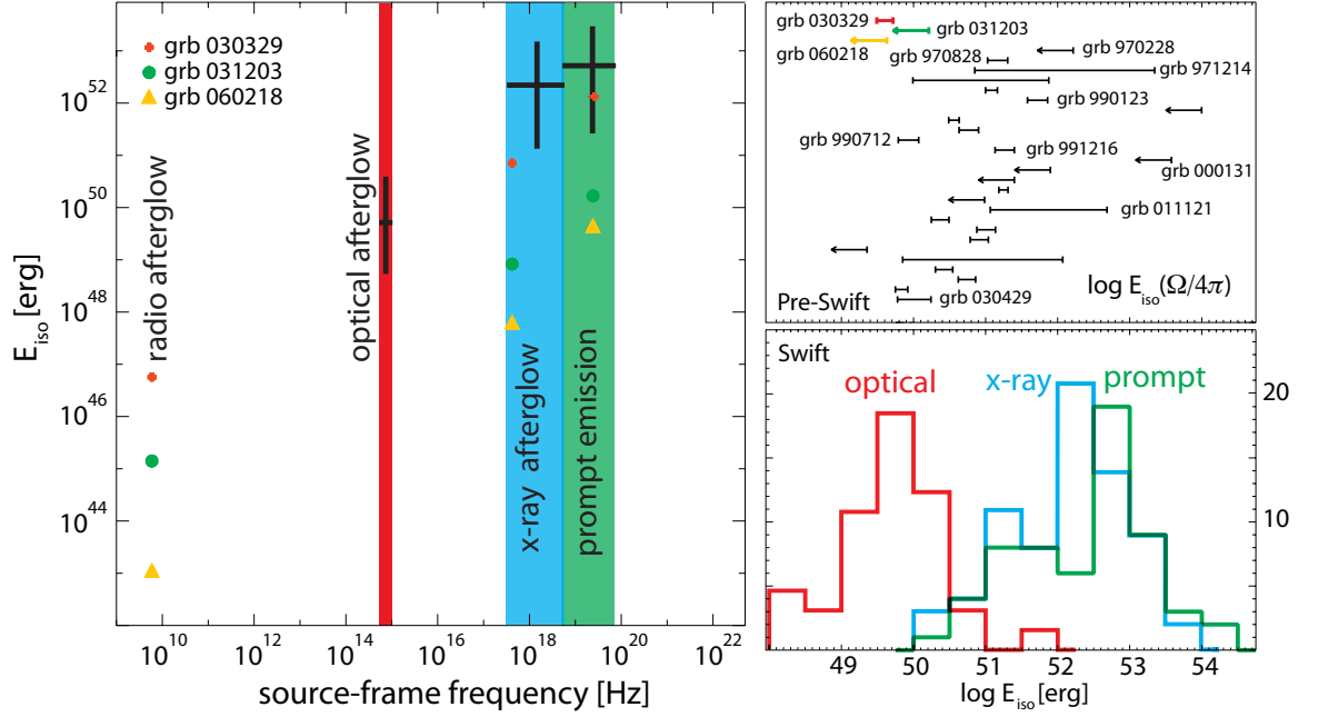
Figure 10 The radiated-energy inventory of Swift GRBs. Left Panel : Summary of the isotropic-equivalent total emitted energy of the prompt and afterglow emission for Swift GRBs in the source frame (adapted from Kaneko et al. 2007). Right Panel Bottom : Distributions of cumulative isotropic-equivalent total emitted energy for Swift GRBs. Right Panel Top : Comparisons of collimation-corrected total emitted \gamma -ray energy, E_{\text{iso}}(\Omega/4\pi) , of pre- Swift GRBs, where E_{\text{iso}} is used as an upper limit for GRBs with no jet angle constraints.
