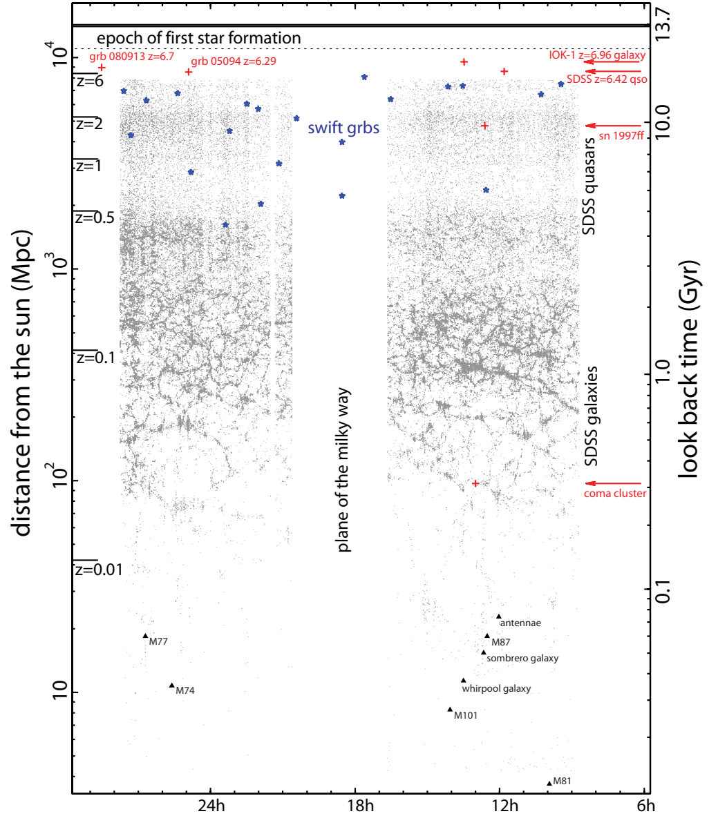
Figure 15 A 360° vista showing the entire sky, with visible structures stretching back in distance, time and redshift. The most distant light we observe comes from the radiation left over from the Big Bang: the CMB. As we descend the chart, we find the most distant objects known, followed by a web of Sloan Digital Sky Survey (SDSS) quasars and galaxies. Closer to home, we start to see a collection of familiar “near” galaxies (triangles). Also marked are all Swift GRBs with known distances (blue stars); SN 1997ff, the most distant type Ia supernova at z = 1.7 ; and the archetypal large galaxy cluster, the Coma cluster. The redshift distances of most distant GRBs are comparable to the most distant galaxies and quasars (adapted from Ramirez-Ruiz 2006a.)
