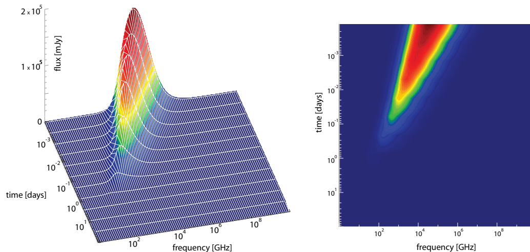
Figure 3 The evolving synchrotron afterglow of a \gamma -ray burst. Shown is a theoretical model (Gou et al. 2007) for the afterglow of the Swift GRB 050904. The model is presented without extinction and as it would have been observed at redshift z = 2 ; the burst itself occurred at z = 6.29 . The evolution of the synchrotron peak to lower frequencies is clearly visible. More subtle effects including evolution of the synchrotron cooling and self-absorption frequencies, and the associated synchrotron self-Compton emission of the blastwave at higher frequencies, are not readily visible in this model.
