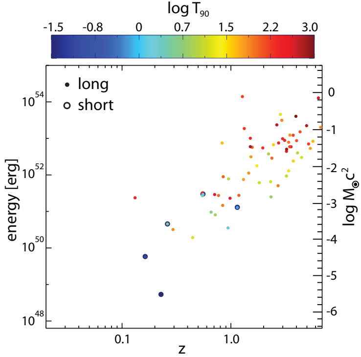
Figure 2 Apparent isotropic \gamma -ray energy as a function of redshift and observed duration. The energy is calculated assuming isotropic emission in a common comoving bandpass for a sample of short and long GRBs with measured redshifts. This spread in the inferred luminosities obtained under the assumption of isotropic emission may be reduced if most GRB outflows are jet-like. A beamed jet would alleviate the energy requirements, and some observational evidence does suggest the presence of a jet.
