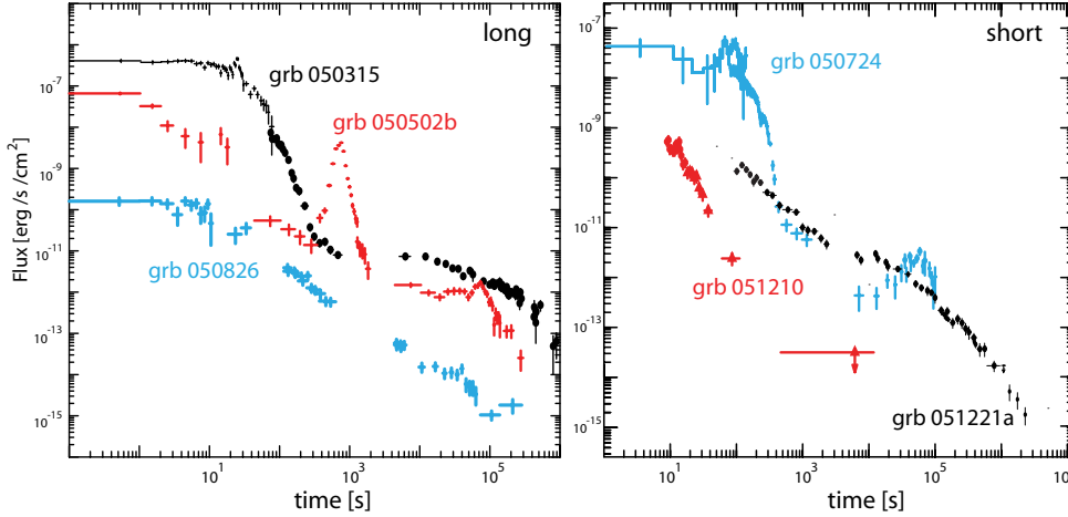
Figure 6 Representative examples of X-ray afterglows of long and short Swift events with steep-to-shallow transitions (GRB 050315, 050724), large X-ray flares (GRB 050502B, 050724), fastly declining (GRB 051210) and gradually declining (GRB 051221a, GRB 050826; flux scale divided by 100 for clarity) afterglows.
