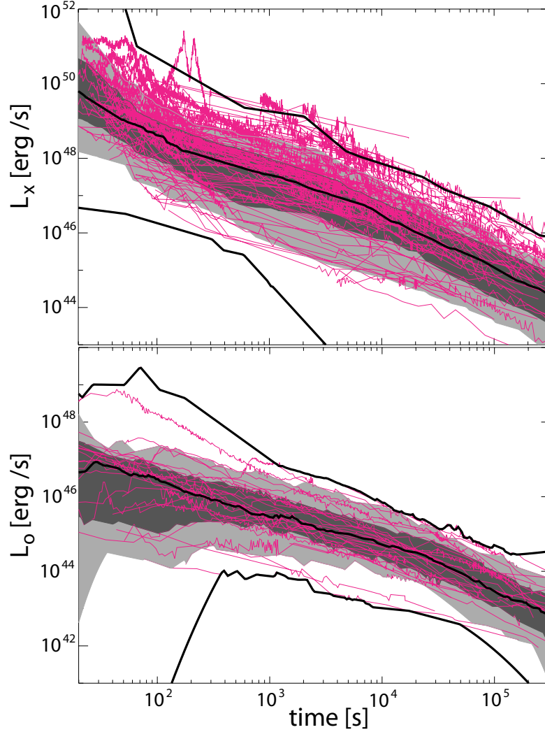
Figure 7 X-ray and optical lightcurves of GRB afterglows in the Swift era. (a) X-ray lightcurves of Swift burst afterglows. Data for long-duration bursts with known redshifts, from GRB050126 to GRB070724A, have been gathered from the Swift XRT lightcurve and spectral data depository at the UK Swift Science Data Centre (Evans et al. 2007; Evans et al. 2008). They are corrected uniformly to unabsorbed luminosity over 1.0 – 30.0 keV in the burst rest-frame, using the time-average afterglow spectrum, and plotted as a function of rest-frame time (pink lines). Separately, afterglow lightcurve fits (Racusin et al. 2008b), which exclude flaring intervals, are used to construct minimum and maximum envelopes (black lines) and confidence intervals (gray bands) on the X-ray luminosities of the bursts as a function of rest-frame time: light gray regions delimit bands of 10% to 90% confidence, dark gray regions delimit bands of 25% to 75% confidence, and the median burst luminosity at any given time is shown (middle black line). (b) Optical lightcurves of Swift burst afterglows. Data for long-duration bursts with known redshifts and at least “bronze” quality published optical data (Kann et al. 2007), from GRB050408 to GRB070612A, are corrected uniformly to rest-frame U -band luminosity using the inferred R -band ( z = 1 ) light-curves from Kann et al. (2007), and plotted as a function of rest-frame time (pink lines). Interpolated and “best fit” extrapolated lightcurves are used to generate minimum and maximum envelopes and median luminosity estimates (black lines) and confidence intervals (gray regions), as in a .
