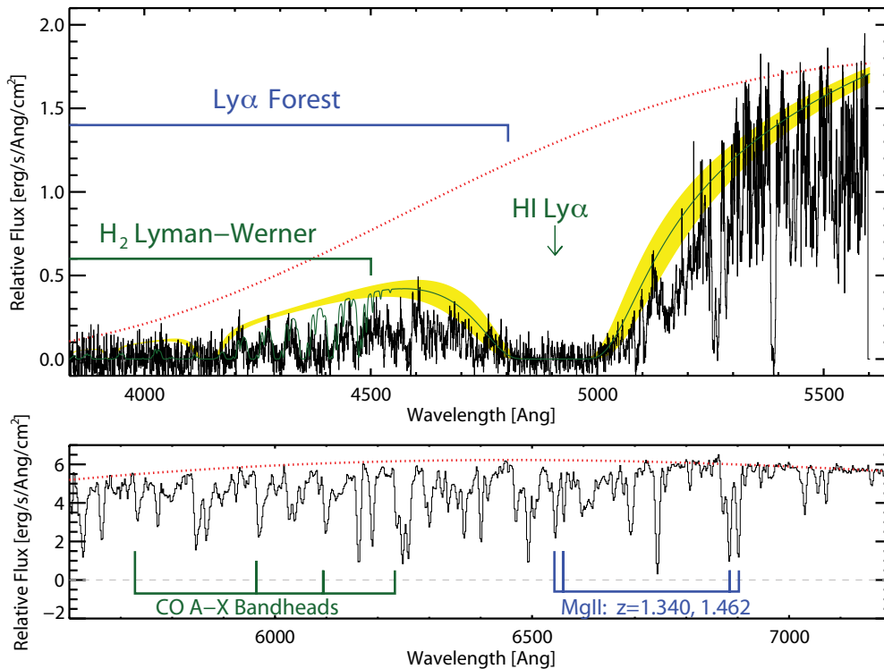
Figure 13 Keck/LRIS spectrum of the afterglow for GRB 080607 (Prochaska et al. 2009). The red dashed lines indicate a model of the intrinsic afterglow spectrum reddened heavily by dust in the host galaxy (rest-frame A_V \approx 3.2 ). At \lambda \approx 4900 Å one identifies a damped Ly \alpha profile associated with H I gas near the GRB. The shaded region overplotted on the data corresponds to an H I column density N_H = 10^{22.7 \pm 0.15} \text{ cm}^{-2} . The model (green solid line) includes absorption from H 2 Lyman-Werner transitions. The line opacity at \lambda > 5500 Å is dominated by metal-line transitions from gas in the host galaxy and includes bandheads of the CO molecule. Surprisingly, this is the only sightline to date to show strong molecular absorption (Tumlinson et al. 2007). It also exhibits a roughly solar metallicity. The figure also shows the spectral region or features corresponding to intergalactic Ly \alpha and MgII absorption. The redshift for GRB 080607 is z = 3.036 .
